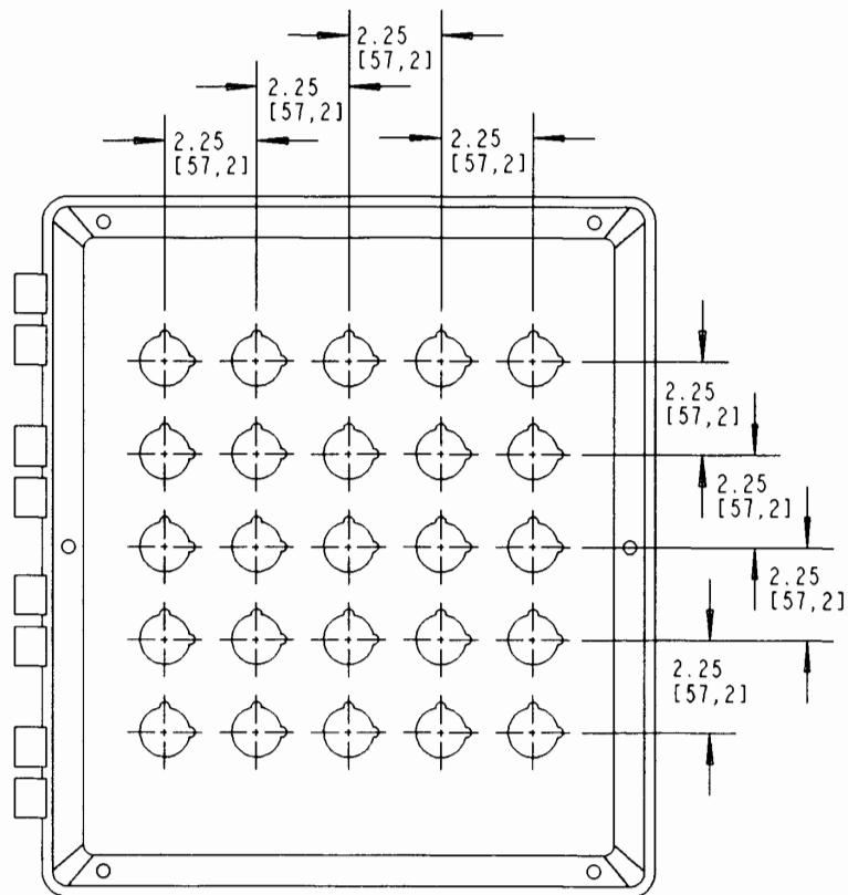
J16147P 25 HOLES
