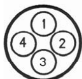
4 WAY BELL END VIEW
